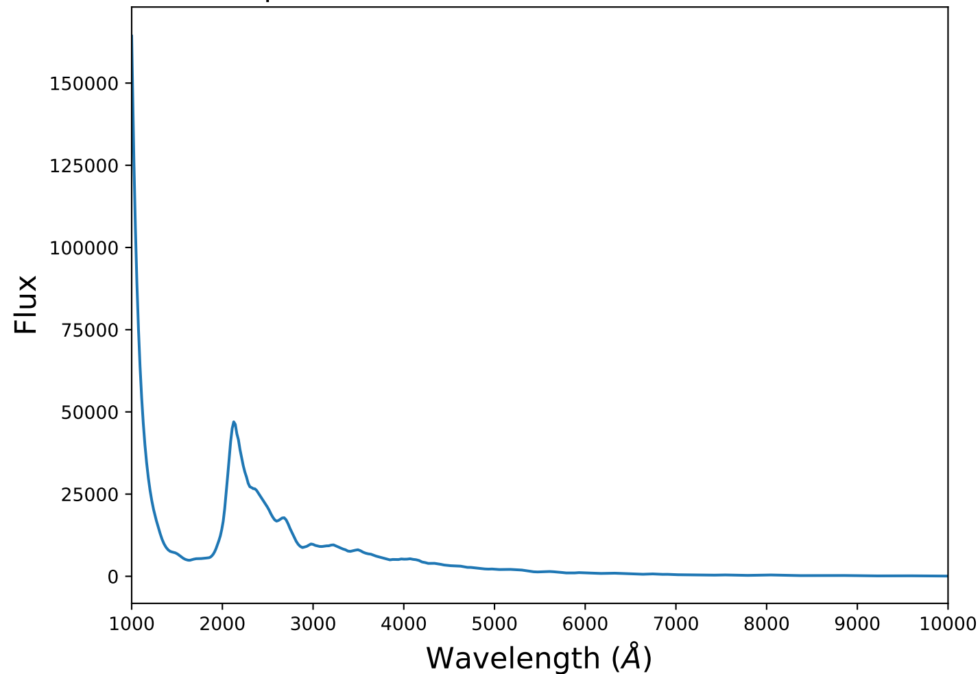
Spectrum 9 for transient SNIa at z=0.46
